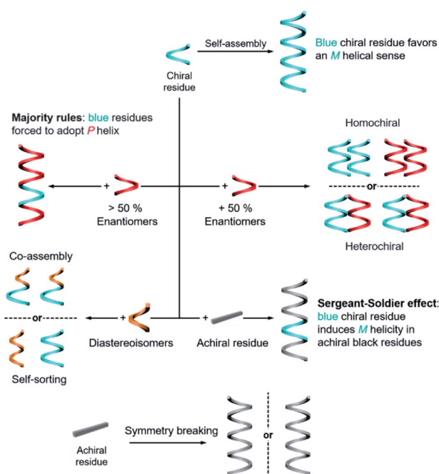
Fig. 3 Fabrication and transmission of chirality during hierarchical self-assembly.
