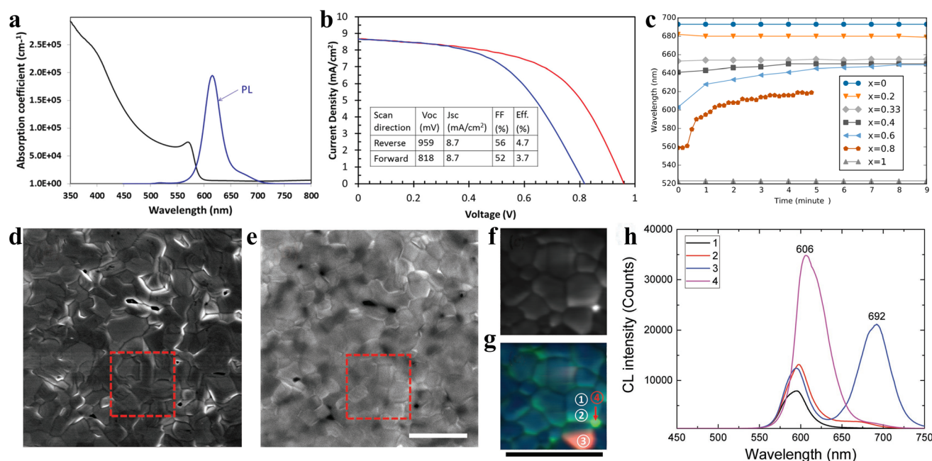
Fig. 8 (a). Absorption coefficient and steady-state PL spectrum of CsPbIBr_2 sample. (b). J-V curves of the best-performing CsPbIBr_2 cell. (a and b) Reproduced with permission. 33 Copyright 2016, Wiley-VCH. (c). PL peak position as a function of time for CsPb(Br_xI_{1-x})_3 materials under ~1 sun illumination. Reprinted with permission. 44 Copyright 2016, the American Chemical Society. (d) Secondary electron SEM image and (e) CL PMT mapping of the CsPbIBr_2 film ( 1024 \times 1024 pixels ( \approx 11 nm on a side); dwell time 50 \mu s per pixel) with the electron beam acceleration voltage of 5 kV and current of 799 pA. The square region in d was further studied by CL spectrum mapping with different spectral windows of 530–630 nm (pixel size of 40 nm \times 40 nm; dwell time of 10 ms). (g). Superposition of (f). (h). CL spectra for the area inside a CsPbIBr_2 grain (GI; region ① in (g)), grain boundary (GB; region ② in (g)), and I-rich phase (areas ③ and ④ in (g)). All the scale bars are 3 \mu m. (d–h) Reproduced with permission. 99 Copyright 2017, Wiley-VCH.
