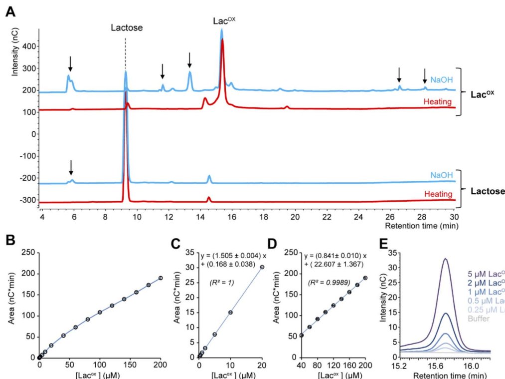
Fig. 4 Features of the HPAEC-PAD LacOX detection method. (A) HPAEC-PAD chromatograms showing the product profile of D-lactose (250 μM final) and LacOX (250 μM final) after treatment with NaOH (0.15 M final; blue lines) or heat (100 °C, 5 min; red lines) (note that the samples were further diluted in water before injection). (B–D) Standard curve of oxidized lactose (LacOX). Panels (C) and (D) show zoom-in views on the [0–20 μM] and [40–200 μM] ranges, respectively. Data points show average values and error bars show standard deviations ( n = 3 independent technical replicates; error bars are <3% of each corresponding average value). (E) Zoom-in view of the HPAEC-PAD chromatogram in the LacOX region showing the detection of very low concentrations.
