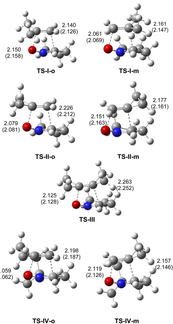
Fig. 3 \omega B97X-D/6-311G(d,p) geometries of the TSs involved in the 32CA reactions of cyclic nitron 21 with MP 22, MCP 11 and DCP 27, and that of cyclic dimethyl nitron 14 with MCP 11. Distances in benzene are given in parentheses. Lengths are given in angstroms.
