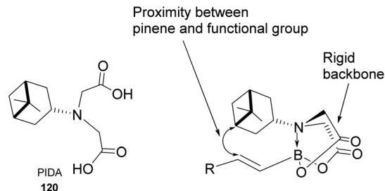
Fig. 11 Pinene-derived iminodiacetic acid (PIDA).
