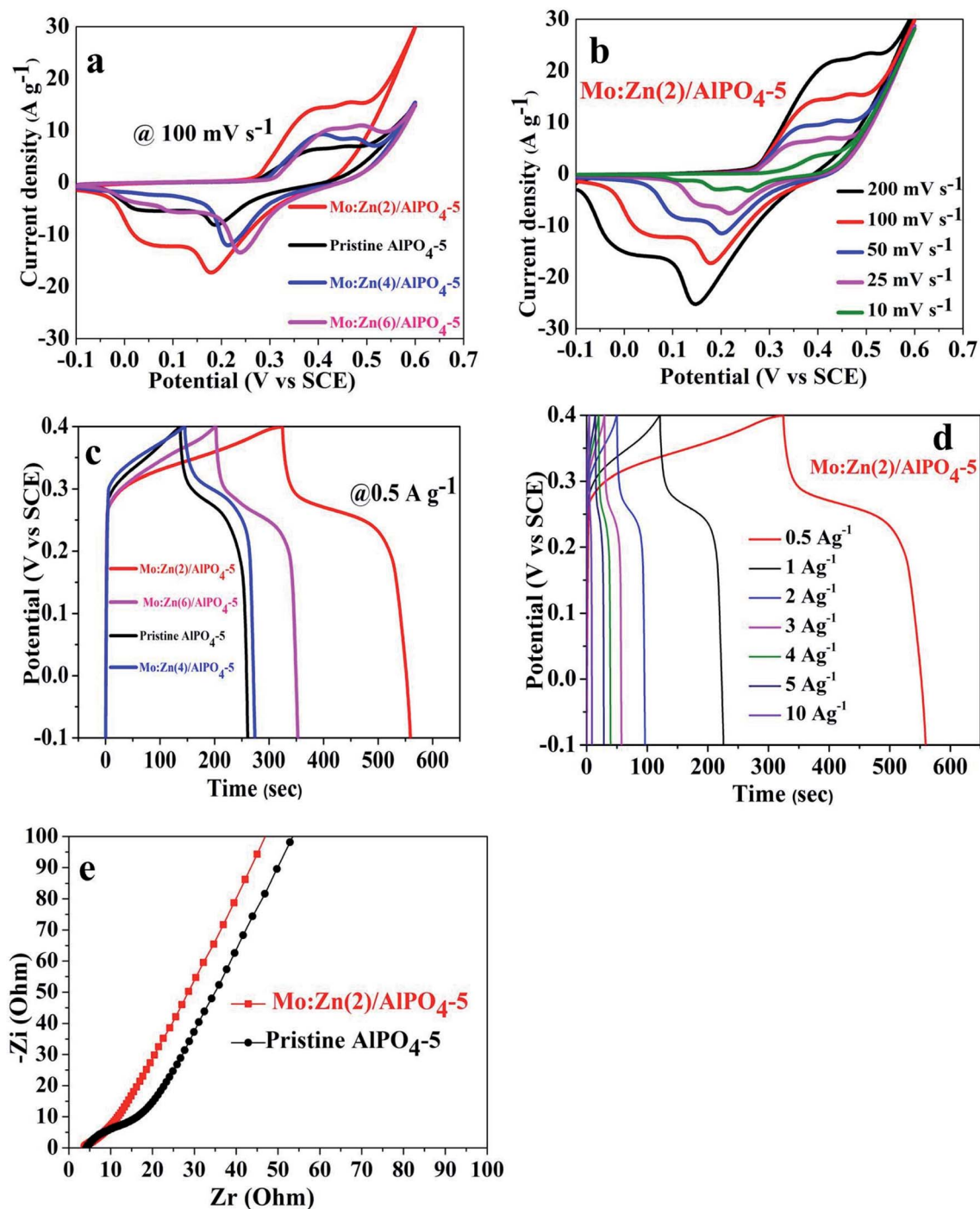
Fig. 13 (a) CV curves of pristine \text{AlPO}_4\cdot 5 and its corresponding Mo, Zn supported \text{AlPO}_4\cdot 5 samples with different mole ratios, (b) CV curves Mo : Zn (2)/ \text{AlPO}_4\cdot 5 at different scan rates, (c) GCD curves of pristine \text{AlPO}_4\cdot 5 and its corresponding Mo, Zn supported \text{AlPO}_4\cdot 5 samples with different mole ratios at 0.5 \text{ A g}^{-1} , (d) CD curves Mo : Zn (2)/ \text{AlPO}_4\cdot 5 at different current densities, and (e) EIS spectrum of pristine \text{AlPO}_4\cdot 5 and Mo : Zn (2)/ \text{AlPO}_4\cdot 5 , respectively.
