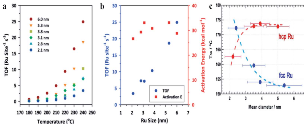
Fig. 5 (a) The turnover frequency (TOF) for the CO to CO 2 oxidation at various temperatures over Ru nanoparticles having different size. (b) The turnover frequency (TOF) for the CO to CO 2 oxidation and the activation energy ( E_a ) of this process at 240 °C over Ru nanoparticles having different size. (c) The temperature for 50% conversion of CO to CO 2 ( T_{50} ) over fcc and hcp Ru nanoparticles having different size. (a) and (b) Reprinted with permission from ref. 2. Copyright 2010 the American Chemical Society. (c) Reprinted with permission from ref. 4. Copyright 2013 the American Chemical Society.
