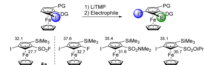
Scheme 4 Top: The 'halogen dance' reaction. Bottom: calculated pK_a values of selected ferrocene derivatives obtained by the 'halogen dance' reaction.
