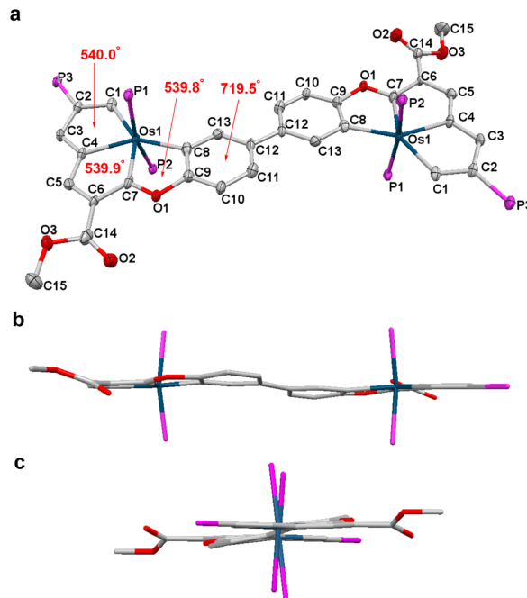
Fig. 1 (a) Crystal structure of 3 ·4CH 2 Cl 2 (thermal ellipsoids set at 50% probability); (b) front view; (c) side view. Hydrogen atoms, BF 4 − counterions, CH 2 Cl 2 molecules and phenyl substituents in PPh 3 have been omitted for clarity. Selected bond lengths (Å) and angles (°) are presented in Table S2 and Fig. S2(a) (ESI † ).
