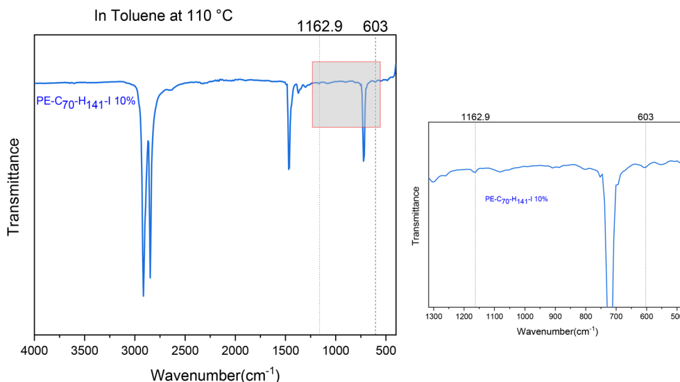
Fig. 5 FT-IR analysis of C_{70}H_{141}I /LDPE polymer blend obtained via solution blending in toluene.
