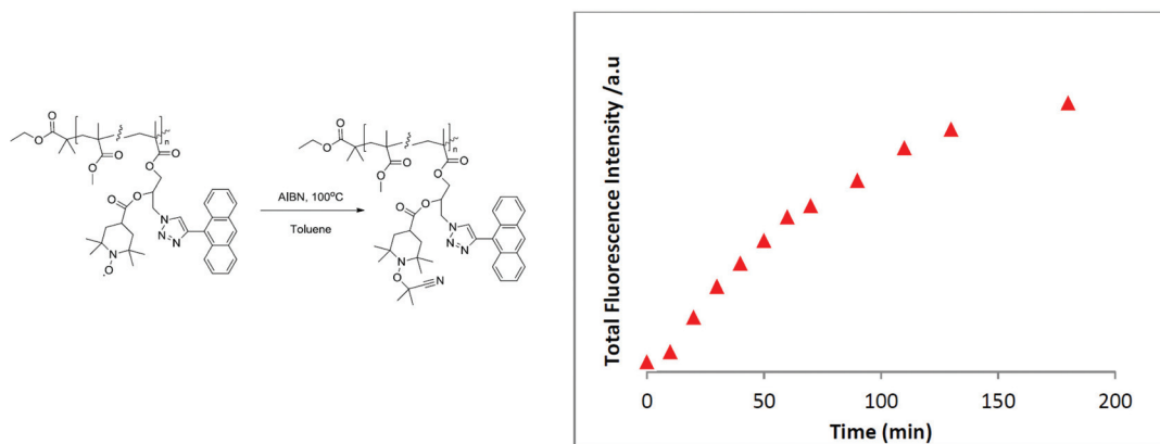
Fig. 1 Evolution of total fluorescence over time when a polymer decorated with an anthracene chromophore and nitroxide moiety is heated at 100 °C in a degassed solution of toluene containing 2.5 equivalents of AIBN. Figure reproduced with permission from ref. 37. Copyright, Royal Society of Chemistry, 2015.
