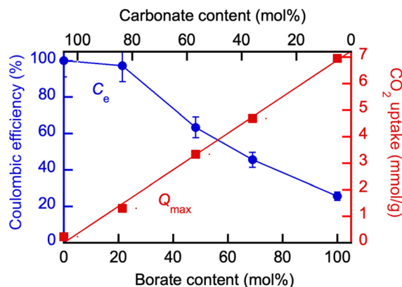
Fig. 12 Effect of the molten borate/carbonate blend composition on the Coulombic efficiency ( C_e ) of the \text{CO}_2 electrolysis and maximum \text{CO}_2 uptake ( Q_{\text{max}} ) at 550 °C. Borate: \text{Li}_{1.5}\text{Na}_{1.5}\text{B}_2\text{O}_3 ; eutectic Li, K carbonate: \text{Li}_{1.24}\text{K}_{0.76}\text{CO}_3 . For Q_{\text{max}} determination detail, see legend to Fig. 6.
