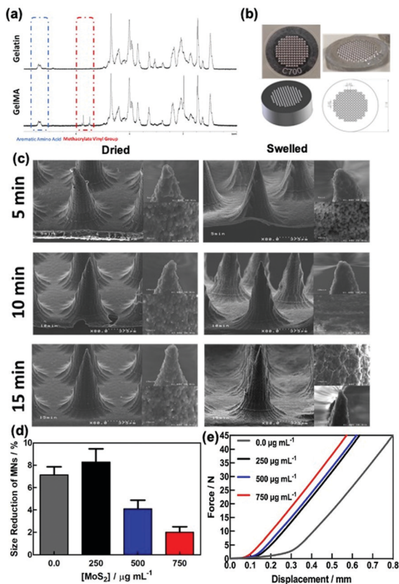
Fig. 2 Morphological characterization of \text{MoS}_2 -MNs: (a) ^1\text{H} NMR of gelatin before and after methacrylation into GelMA. (b) Photographs of MN aluminum master molds from different perspectives. (c) SEM images of the \text{MoS}_2 loaded MN array using 300 \mu\text{L} of a hydrogel cocktail of GelMA : PEDGMA (20 : 10) (2 mL) and 1.0 mg \text{MoS}_2 , polymerized using different UV irradiation times. (d) Influence of \text{MoS}_2 content (250, 500 and 750 \mu\text{g mL}^{-1} ) in the hydrogel cocktail on the mechanical strength of MN hydrogel arrays. (e) Force–displacement curves recorded for GelMA : PEDGMA (20 : 10) hydrogel MNs without and with increasing \text{MoS}_2 content (250, 500 and 750 \mu\text{g mL}^{-1} ) in the polymerization mixture.
