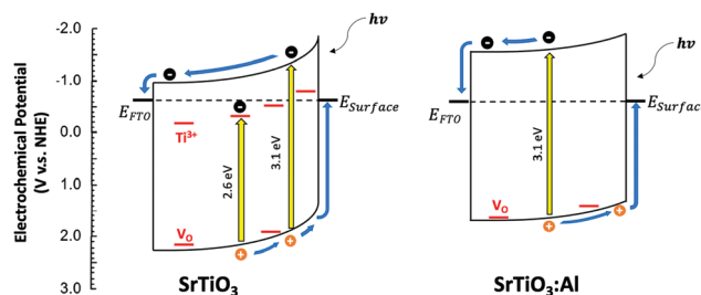
Fig. 12 Charge transfer and energetics during the SPV experiment for V O rich SrTiO 3 and Al-doped SrTiO 3 (heating 1). In SrTiO 3 :Al, Ti 3+ trap states were eliminated by Al 3+ doping, leading to a less reducing Fermi level, fewer trapped electrons, and less band bending. The lower band bending in SrTiO 3 :Al is indicated by the lesser surface photovoltage signal. E Surface denotes the energy of surface states resulting from dangling bonds, reduced ions, or surface adsorbates. Ti 3+ and V O lattice defects (shown in red) are responsible for the sub-band gap photovoltage signal. E FTTO is the Fermi level of the fluorine doped tin oxide substrate.
