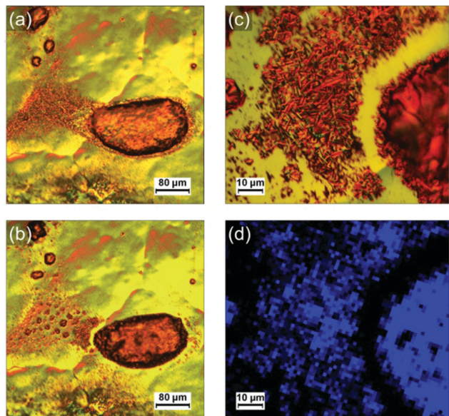
Fig. 3 Optical micrographs of the mixture (diluted 100 times) deposited on HOPG (a) before and (b and c) after irradiation during 3 min at 405 nm. Image (c) corresponds to a zoomed-in region from (b). (d) Raman map of the density of polymerized blue PDA (i.e. intensity value of the Raman peak at \approx 2080\text{ cm}^{-1} ). Map in (d) corresponds to the same region as in (c) after UV irradiation for 20 s. Color code: black = no PDA, blue = PDA.
