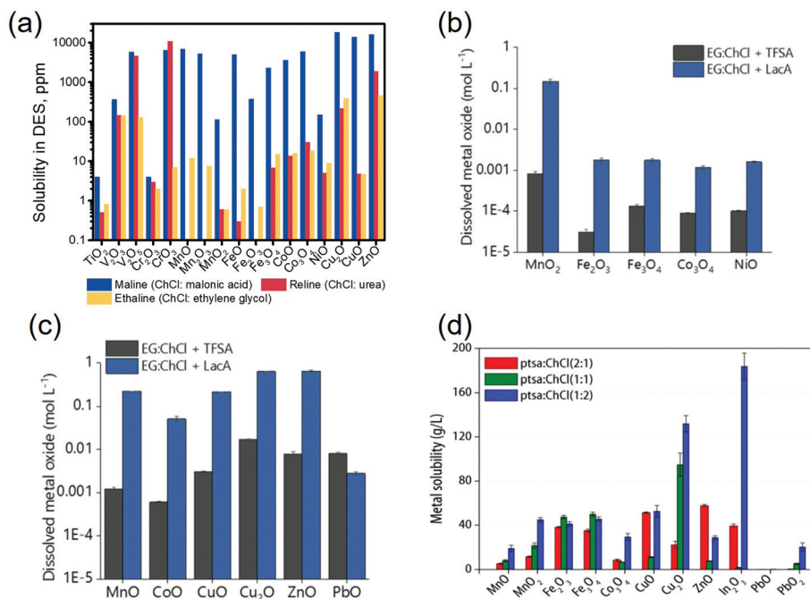
Fig. 5 Solubility of metal oxides in various DESs. (a) Solubility of metal oxides in maline (ChCl: malonic acid, 1:1), reline (ChCl: urea, 1:2), and ethaline (ChCl: ethylene glycol, 1:2) at 50 °C after 2 days. Reproduce with the data from ref. 116. Copyright © 2006, American Chemical Society. (b and c) Solubility of metal oxides in ChCl: ethylene glycol (EG) with either 10 -3 M trifluoromethanesulfonic acid (TFSA) or with lactic acid (LacA) at 50 °C after 2 days: (b) less soluble oxides, (c) more soluble oxides. Reprint with the permission from ref. 129. Copyright © 2020, Royal Society of Chemistry. (d) Solubility of metal oxides in p -toluenesulfonic acid monohydrate (PTSA): chlorine chloride (ChCl) DESs at different HBD:HBA molar ratio at 50 °C. Reprint with permission from ref. 70, Copyright © 2019, American Chemical Society.
