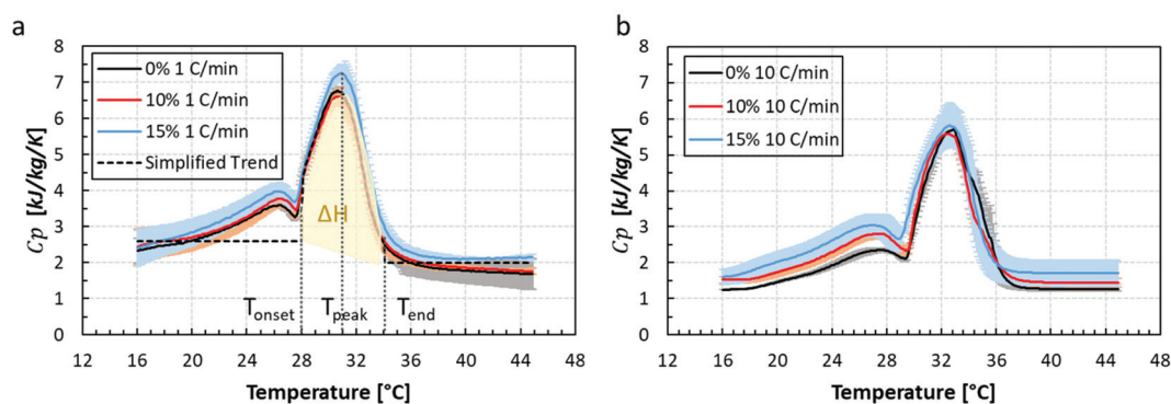
Fig. 6 DSC data for all types of chocolates at two different heating rates, 1\text{ °C min}^{-1} (a) and 10\text{ °C min}^{-1} (b). The dashed line in (a) shows the simplified version of the C_p trend used as an initial input for the numerical model. The dotted lines indicate the location of T_{\text{onset}} , T_{\text{peak}} , T_{\text{end}} .
