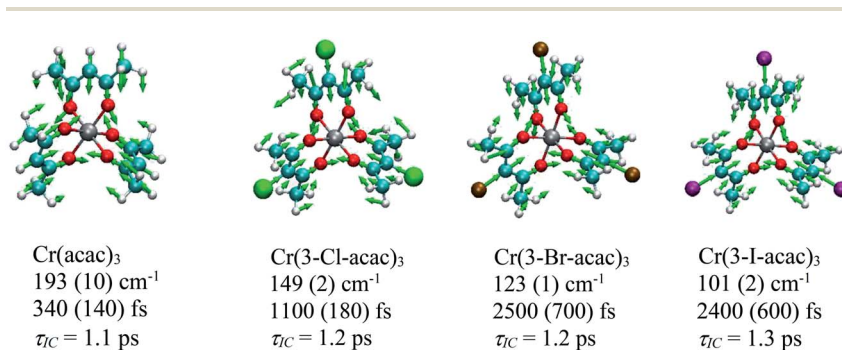
Fig. 13 Nuclear displacements associated with the coherent oscillations identified for the \text{Cr(3-R-acac)}_3 derivatives. Below each compound's name is listed the DFT calculated frequency associated with the coherence feature, the measured dephasing time, and the time constant corresponding to the observed kinetics for excited-state evolution based on the model shown in Fig. 9.
