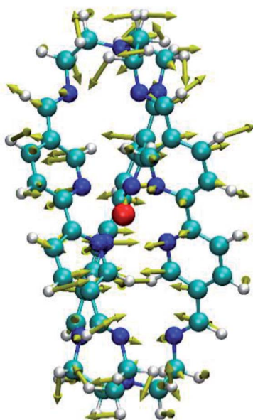
Fig. 6 DFT-based vector displacement diagram of the 154 \text{ cm}^{-1} mode identified from the LPSVD analysis of the data plotted in Fig. 5. The large-amplitude motion of the ligand framework evident above and below the \text{Fe}(\text{II}) coordination site (red) was targeted for chemical modification via binding to \text{Cu}(\text{I}) .
