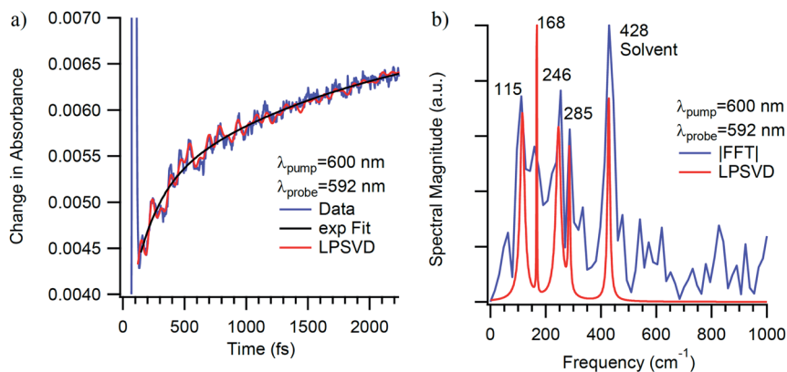
Fig. 14 Ultrafast time-resolved absorption data for \text{Cr(TMHD)}_3 in a 1,4-dioxane solution. (a) Single-wavelength kinetics data acquired at 592 nm following ca. 40 fs excitation into the ^4A_2 \rightarrow ^4T_2 ligand-field absorption band at 600 nm. The blue line corresponds to the experimental data, the black line a fit of the population dynamics to a single exponential kinetic model, and the red to the results of an LPSVD analysis. (b) LPSVD (red) and FFT (blue) analysis of the quantum oscillations observed in the experimental data shown in part (a). Features appearing at 115 \text{cm}^{-1} , 168 \text{cm}^{-1} , and 246 \text{cm}^{-1} correspond to the three vibrational signatures that were consistently observed across variations in solvent as well as pump/probe wavelength combinations.
