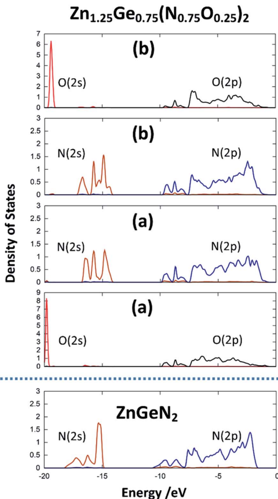
Fig. 7 pDOS for the 2s and 2p orbitals for one selected nitrogen and oxygen atom in the crystal structures for \text{ZnGeN}_2 and the two configurations of \text{Zn}_{1.25}\text{Ge}_{0.75}(\text{N}_{0.75}\text{O}_{0.25})_2 , as depicted in Fig. 2.
