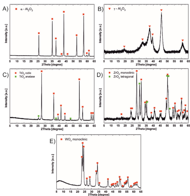
Fig. 3 X-ray diffractograms of the crystalline inorganic fibers: A) \text{Al}_2\text{O}_3 \alpha , B) \text{Al}_2\text{O}_3 \gamma , C) \text{TiO}_2 rutile, D) \text{ZrO}_2 , and E) \text{WO}_3 .
