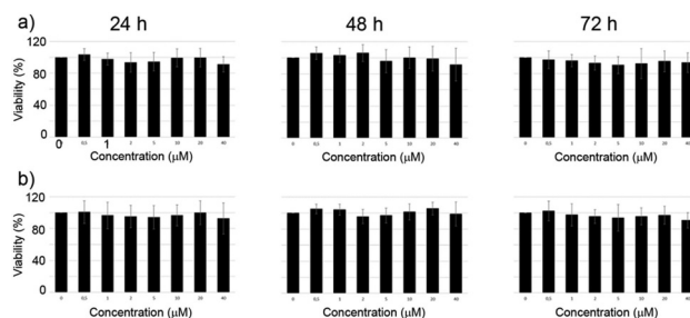
Fig. 8 Cellular viability of M21 cells after treatment with increasing amounts of: (a) [Eu(L 1 )] 3+ and (b) [Eu(L 2 )] 3+ (from MTT assays). The results were expressed as a percentage of the vehicle treated cells. Data shown are the mean \pm SD of three independent experiments. The concentrations are 0, 0.5, 1, 2, 5, 10, 20, 40 \mu M from the first to the last column for each graph.
