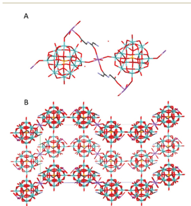
Fig. 6 The molecular (A) and crystal (B) structure of compound Na(HGlyGly)(H 3 O)[PMo 12 O 40 ] \cdot 3H 2 O (6).
