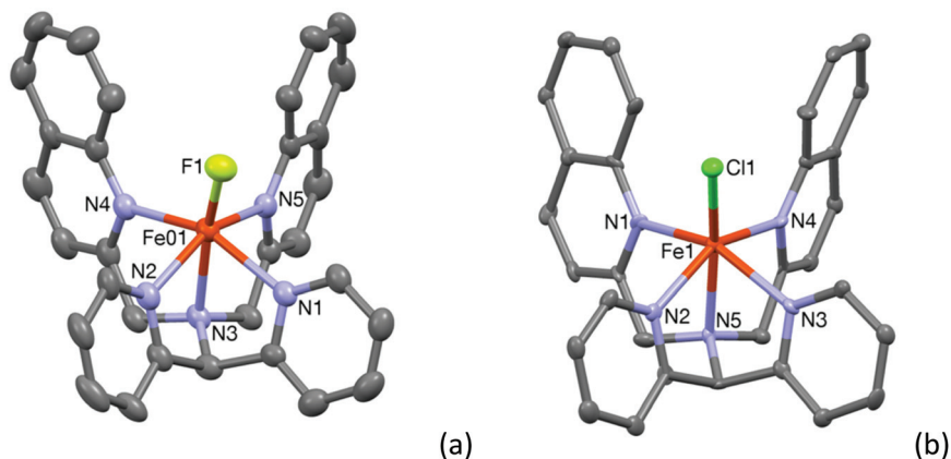
Fig. 1 Mercury plots of the molecular structures of the cationic complexes 1 (a) and 2 (b), showing the atom labelling scheme. Thermal ellipsoids are plotted at 30% probability ellipsoids; hydrogen atoms have been omitted for clarity.
