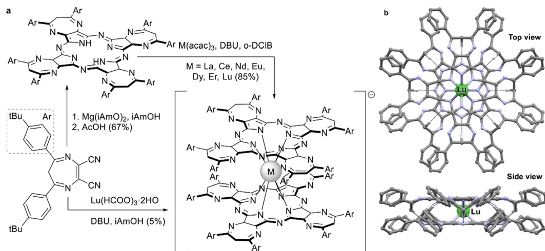
Scheme 26 (a) Synthesis of double-decker complexes with tetradiazepinoporphyrazine ligands. (b) Optimized structure of Lu(Ph_8DZPz)_2 in top and side views, showing hydrogen bonds between CH_2 groups of diazepine rings and meso -N atoms. Other hydrogen atoms are omitted for clarity. Model was built using Cartesian coordinates, provided in the ESI in ref. 143.
