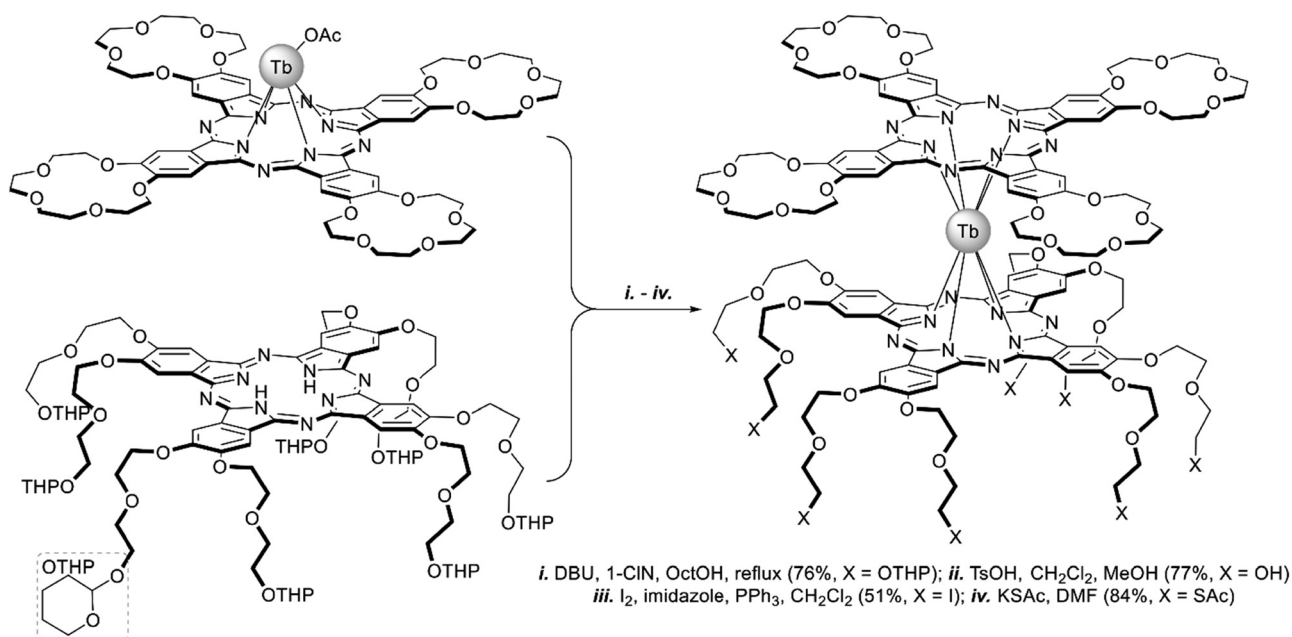
Scheme 4 Synthesis of heteroleptic octopus-type \text{Tb(III)} bisphthalocyanine. 73
