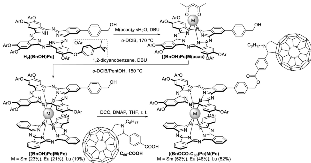
Scheme 17 Synthesis of fullerene-substituted bisphthalocyaninates [(\text{BnOCO-C}_{60})\text{Pc}]\text{M}(\text{Pc}) . 118
