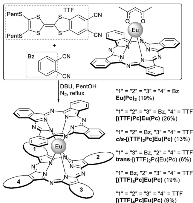
Scheme 18 One-pot synthesis of a series of tetrathiafulvalene (TTF)-fused bisphthalocyaninates [(\text{TTF})_n\text{Pc}]\text{Eu}(\text{Pc}) , n = 0-4 . 118
