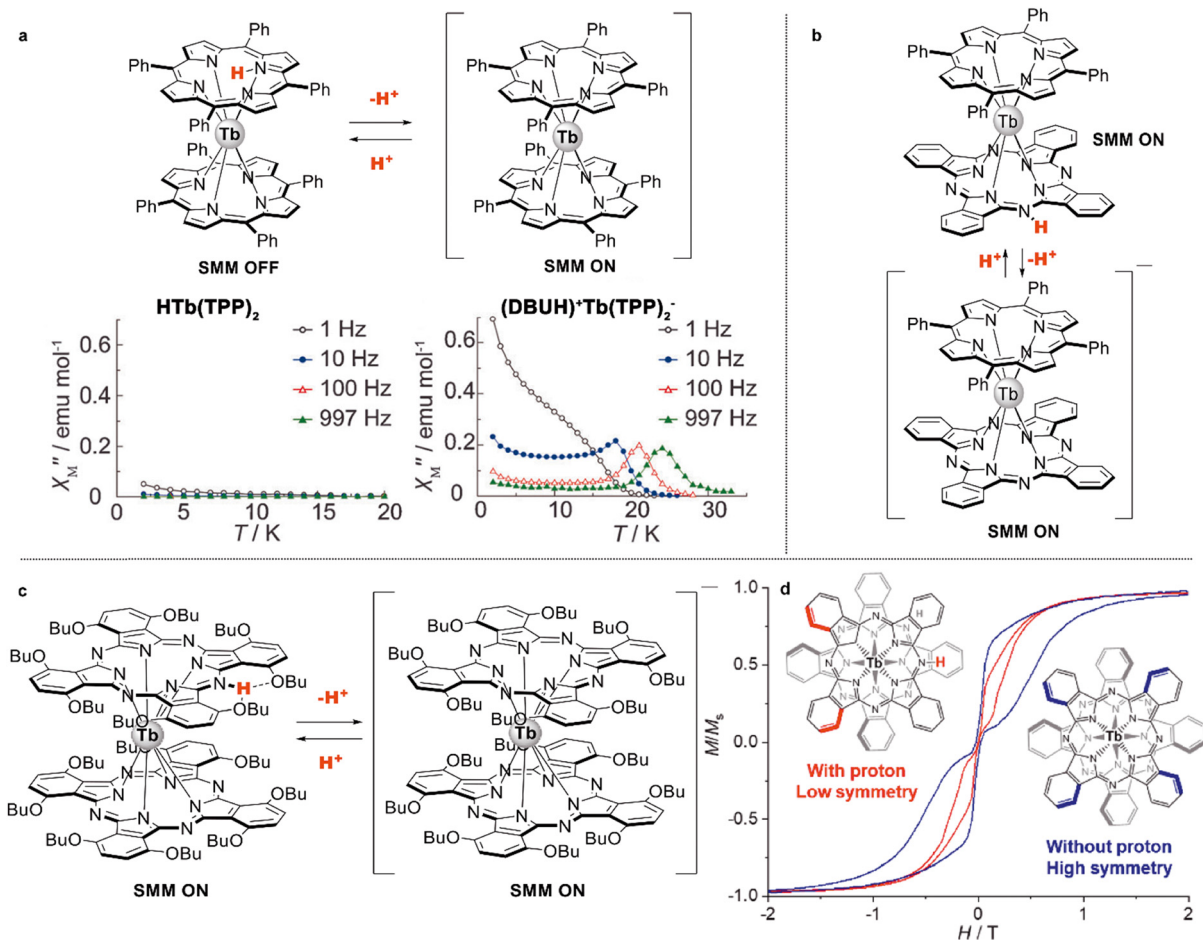
Fig. 28 (a) Proton-induced on/off switching of SMM properties ( \text{HTb(TPP)}_2 and (\text{HDBU}^+)\text{Tb(TPP)}_2^- ). (b) Protonation/deprotonation of the porphyrinato-phthalocyaninato \text{Tb}^{3+} double-decker complex \text{HTb}(\alpha\text{-BuO})_8\text{Pc}]_2 and (c) phthalocyaninato-phthalocyaninato double-decker complex \text{HTb}(\alpha\text{-BuO})_8\text{Pc}]_2 . (d) Magnetic hysteresis curves of the protonated ( \text{HTb}(\alpha\text{-BuO})_8\text{Pc}]_2 ) and deprotonated form ( (\text{HDBU}^+)\text{Tb}(\alpha\text{-BuO})_8\text{Pc}]_2^- ) of the double-decker complex. Reproduced from (a) ref. 297 with permission from the Royal Society of Chemistry. Adapted with permission from (d) ref. 97. Copyright 2018, American Chemical Society.
