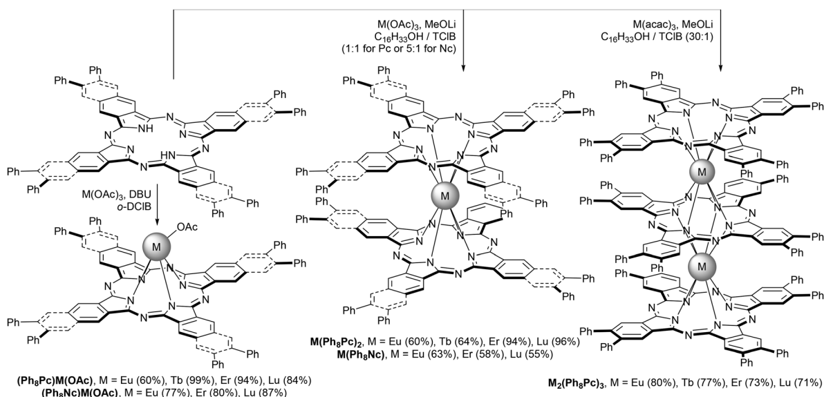
Scheme 2 Synthesis of lanthanide complexes with phenyl-substituted phthal- and naphthalocyanines. 50,51
