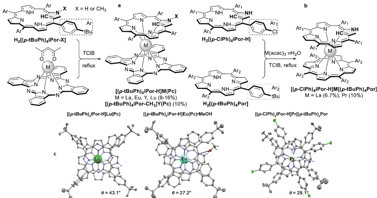
Scheme 31 (a and b) Synthesis of heteroligand double-decker complexes with N -confused ligands. (c) X-ray structures of [(tBuPh)_4iPorH]Lu(Pc) (CCDC YEFZIU), [(tBuPh)_4iPorH]Eu(Pc) \cdot MeOH (CCDC YEFZAM) 171 and [(p-ClPh)_4iPorH]Pr[(tBuPh)_4Por] (CCDC BODFIL). 172 Solvate molecules and most of hydrogen atoms are not shown for clarity.
