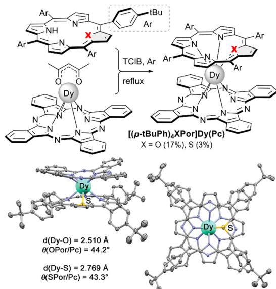
Scheme 32 Synthesis of mixed ligand double-decker complexes with oxa- and thiaporphyrin ligands and X-ray structure of [(tBuPh)_4SPor]Dy(Pc) (CCDC AHOPUK). 173 Hydrogen atoms and solvent molecules are not shown for clarity.
