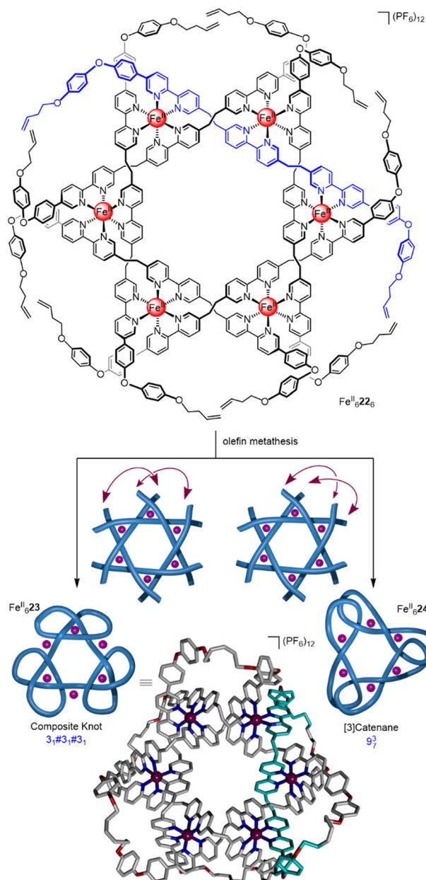
Fig. 8 A hexameric circular helicate and its closure to give molecular composite knot \text{Fe}^{\text{II}}_{23} and link \text{Fe}^{\text{II}}_{24} . 58
