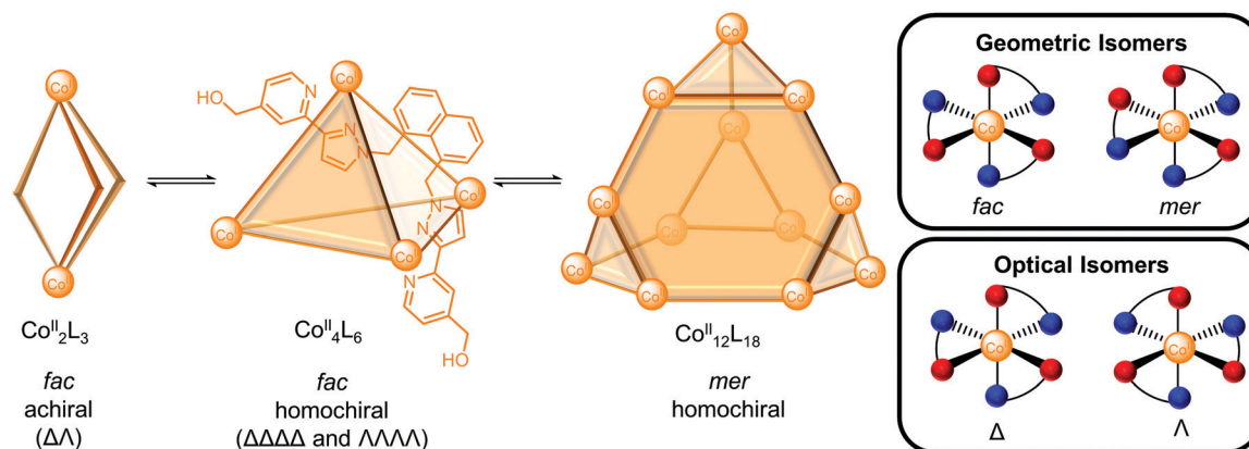
Fig. 2 Mixture of a \text{Co}_2\text{L}_3 meso-helicate, \text{Co}_4\text{L}_6 tetrahedron and \text{Co}_{12}\text{L}_{18} truncated tetrahedron reported by Ward and co-workers where the three architectures result from stereoisomerism of the metal complexes. Inset: Schematic representation of the geometric and optical isomers of individual metal centres where the red and blue balls represent pyridyl and pyrazoyl donor atoms of the cage ligand, respectively.
