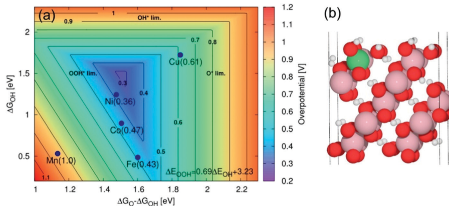
Fig. 42 (a) 2D map of theoretical overpotentials \eta for the doped 1014 surface of \beta -CoOOH as function of \Delta G_O - \Delta G_{OH} and \Delta G_{OH} . The individual values of \eta are indicated in brackets. Improvement in activity relative to undoped surface is obtained in the case of Ni with \eta = 0.36 V and Fe with 0.43 V. Reproduced with permission from ref. 711. Copyright American Chemical Society 2013.
