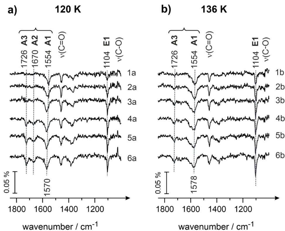
Fig. 4 IR spectra of butanal adsorbed on Pd(111) at (a) 120 K and (b) 136 K at different butanal exposures. Butanal was dosed with a flux of 3.7 \times 10^{12}\text{ mol cm}^{-2}\text{ s}^{-1} resulting in exposures of (1a and 1b) 1.9 \times 10^{14} , (2a and 2b) 2.6 \times 10^{14} , (3a and 3b) 4.1 \times 10^{14} , (4a and 4b) 5.6 \times 10^{14} , and (5a and 5b) 7.8 \times 10^{14}\text{ mol cm}^{-2} . Spectra (6a and 6b) were obtained during continuous butanal dosing via the molecular beam resulting in an overall exposure of 22.0 \times 10^{14}\text{ mol cm}^{-2} .
