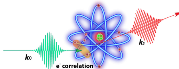
Fig. 1 Schematic illustration of the importance of electron correlation in X-ray scattering, with \mathbf{k}_0 and \mathbf{k}_s being the incoming and outgoing wave vectors of the incident and scattered X-ray photons, respectively. See Section 2.1 for details.
