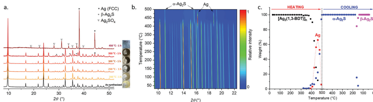
Fig. 2 (a) Normalized intensities of RT PXRD patterns ( \lambda = 1.54056 Å) of ex situ calcinations of [Ag_2(1,3-BDT)]_n for one hour in air at 200, 250, 300, 350 and 450 °C. On the right, the photos of the sample after their calcinations. (b) 2D map of relative intensities of in situ PXRD ( \lambda = 0.67122 Å) of [Ag_2(1,3-BDT)]_n with temperature from RT to 500 °C at 10 °C min -1 in air and (c) weight percentages of the different phases ( [Ag_2(1,3-BDT)]_n (black), Ag (red), \alpha - Ag_2S (blue) and \beta - Ag_2S (pink)) present upon heating and cooling.
