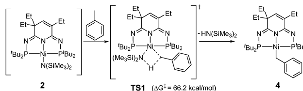
Scheme 3 Calculated toluene activation pathway by complex 2 .
