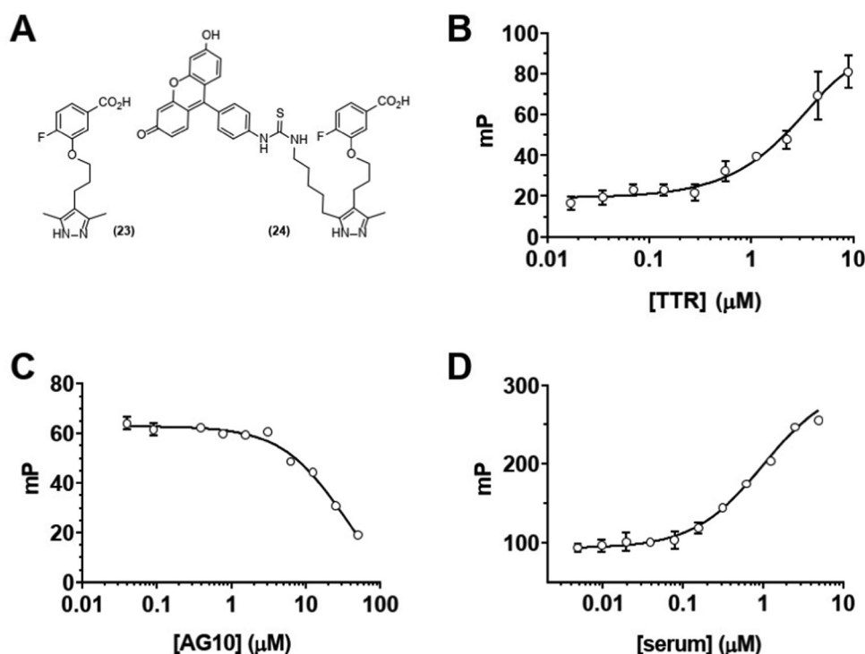
Fig. 1 Analogs of AG10 ( 23 ) and GD10 ( 24 ) bind to TTR and serum proteins. (A) Chemical structures of TTR ligands. (B) Direct binding of ligand 24 to TTR (0.017–9 μM) in buffer by FP ( k_{\text{app}} = 5 \mu\text{M} ); (C) competition of the 24 -TTR complex with increasing concentrations (0.04–50 μM) of AG10 analog 23 ( k_{\text{app}} = 30 \mu\text{M} ); (D) binding of compound 24 to mouse serum proteins (0.005–5 μM) ( k_{\text{app}} = 1 \mu\text{M} ).
