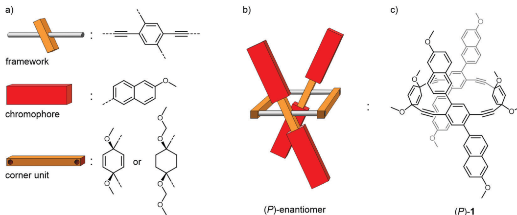
Fig. 2 (a) The molecular subunits representing the functional building blocks. (b) Conceptual picture of the ( P )-enantiomer and (c) its realization with the molecular subunits using 1,4-cyclohexadiene corner units resulting in the target structure ( P )-1.
