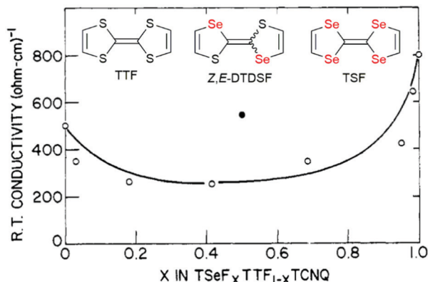
Fig. 4 Room temperature conductivity of (TSF) x (TTF) 1-x (TCNQ) (open circles). The closed black circle refers to [(Z,E)-DTDSF](TCNQ) (see text). Adapted from ref. 34. © 1977 American Chemical Society.
