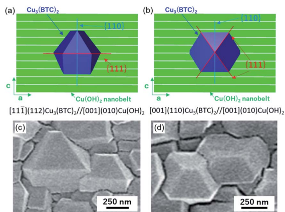
Fig. 2 Schematics and SEM images of the \text{Cu}_3(\text{BTC})_2 crystals epitaxially grown under [11\bar{1}](112)\text{Cu}_3(\text{BTC})_2//[\text{001}](010)\text{Cu}(\text{OH})_2 (a and c) and [\text{001}](110)\text{Cu}_3(\text{BTC})_2//[\text{001}](010)\text{Cu}(\text{OH})_2 (b and d) orientation relationships. The cuboctahedron-shaped crystals and green rectangles denote the \text{Cu}_3(\text{BTC})_2 crystals and \text{Cu}(\text{OH})_2 nanobelts, respectively. In the SEM images, the longitudinal direction ( a -axis) of the underlying \text{Cu}(\text{OH})_2 nanobelts is aligned horizontal to the images.
