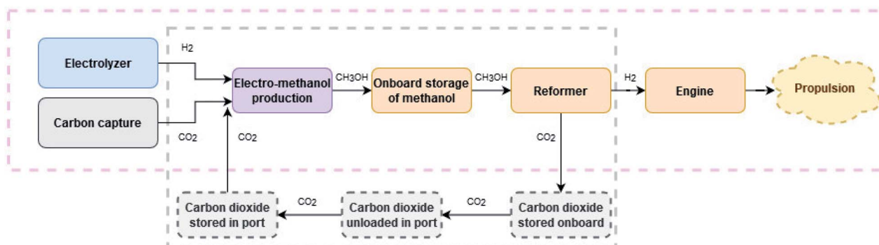
Fig. 1 Outline of the HyMethShip concept. The HyMethShip concept combines a reformer, storage systems for CO 2 and methanol, as well as an ICE into one system ( www.hymethship.com ). Hydrogen produced from an electrolyzer is used together with captured carbon to produce methanol. The produced electro-methanol is used as a hydrogen carrier stored on the vessel until required for propulsion. A reformer splits the methanol into hydrogen, which is used to propel the vessel, and carbon dioxide, which is captured and liquified, brought to shore and utilized in the electro-methanol production. The orange colored processes occur onboard the vessel. The pink system boundary shows the main processes included in this work and the grey system boundary marks the re-circulated CO 2 .
