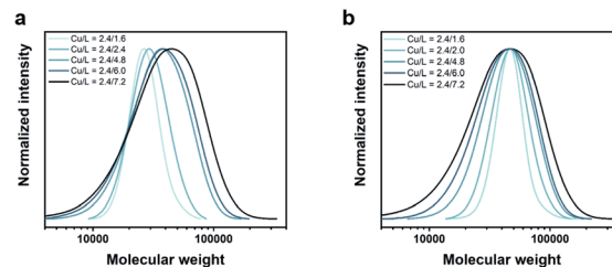
Fig. 1 Tuning the dispersity of PNIPAM in water using different [\text{Cu}^{\text{I}}\text{Br}] : [\text{Me}_6\text{Tren}] ratios while maintaining constant (a) target DP and (b) M_p .
