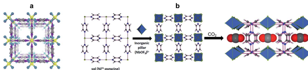
Fig. 1 MOFs/HUMs for DAC by physisorption. (a) Crystal structure of SIFSIX-3-Ni. (b) Crystal structure of NbOFFIVE-1-Ni and binding of CO 2 in its pores. Adapted with permission from ref. 20. Copyright (2016) American Chemical Society.
