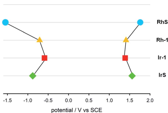
Fig. 5 Diagram of the redox potentials ( E_{1/2} or E_{pa} at 0.5 V s -1 in CH 2 Cl 2 relative to SCE) of RhS (light-blue circle), Rh-1 (yellow triangle), Ir-1 (red square) and IrS (green diamond).
