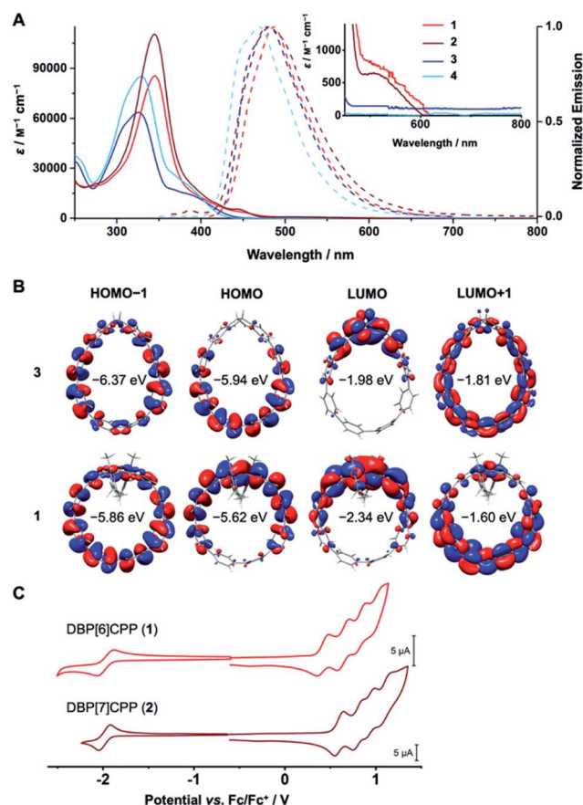
Fig. 4 (A) Absorption ( 10^{-5} to 10^{-6} M) and emission spectra ( 10^{-6} to 10^{-7} M) of 1–4 in \text{CH}_2\text{Cl}_2 ; (B) frontier molecular orbitals of 3 and 1 (PW6B95–D3(BJ)/def2-QZVPP//PBEh–3c); (C) cyclic voltammograms of 1 and 2 (negative potential range in THF, positive in \text{CH}_2\text{Cl}_2 , 1 mM concentration, 0.1 M n\text{-Bu}_4\text{NPF}_6 , scan rate 0.2 \text{ V s}^{-1} , glassy carbon electrode, potentials plotted vs. \text{Fc}/\text{Fc}^+ as internal standard).
