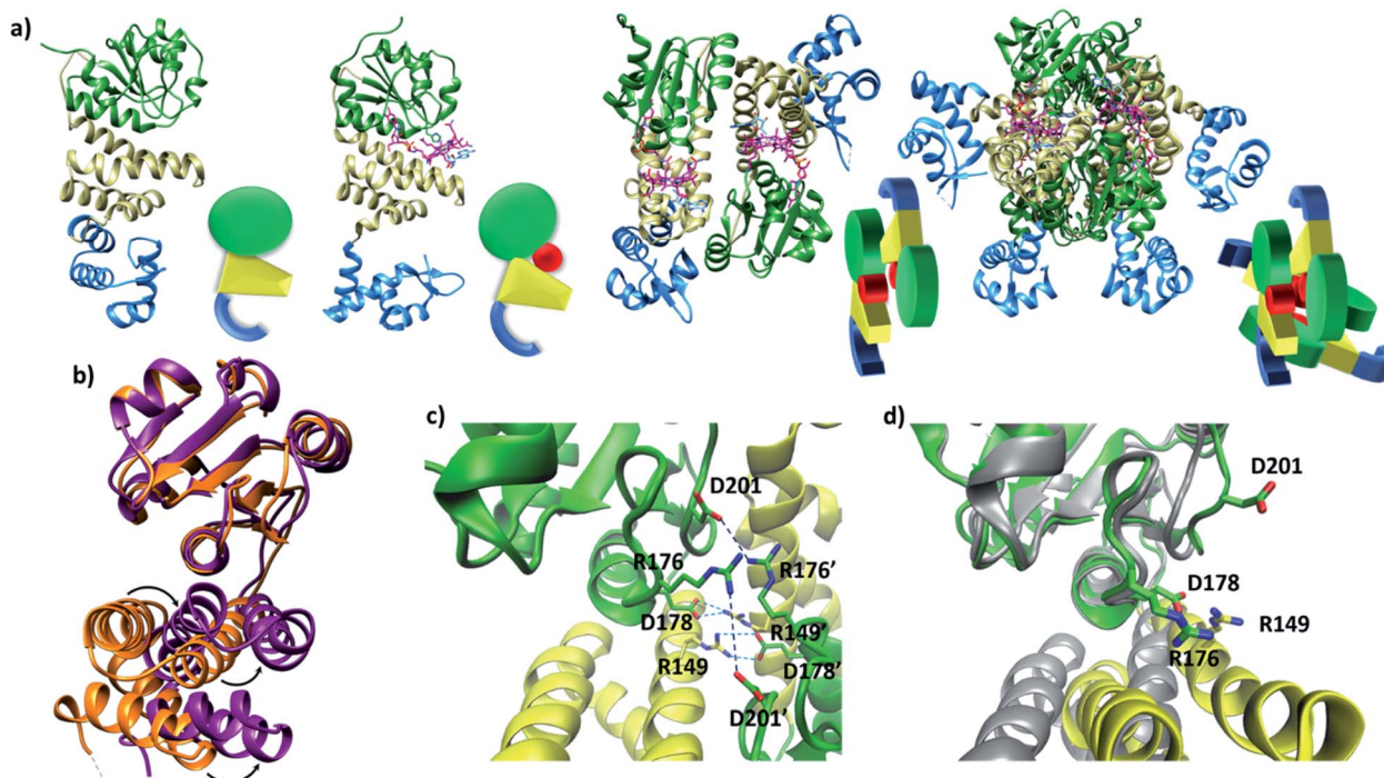
Fig. 1 (a) TtCarH structures and their cartoon representations, colored by their domain: B_{12} -binding (green), 4-helix bundle (yellow), DNA-binding (blue), and AdoCbl (magenta). L–R: apo-monomer (representative from MD simulations), holo-monomer, holo-dimer, and holo-tetramer (all PDB: 5C8D). (b) 4-helix bundle (bottom) positions in each monomer aligned to the B_{12} -binding domain (top): holo-TtCarH (orange, PDB: 5C8D) and apo-TtCarH (purple, simulated). A different color scheme to panel (a) is used to distinguish between different structures. Arrows indicate helical displacement in apo-TtCarH relative to holo-TtCarH (see also Fig. S3a and b†). (c) Close-up of the interface between monomer units in the holo-TtCarH head-to-tail dimers with salt-bridges identified here (D178–R149) and previously 10 (D201–R176) highlighted. (d) The same interfacial region illustrated in panel (c), but now of the simulated apo-TtCarH monomer. The change in 4-helix bundle conformation relative to holo-TtCarH (in grey) results in a helix moving into the dimer interface such that the key salt-bridge residues are no longer able to stabilize the head-to-tail dimers (see also Fig. S3c†).
