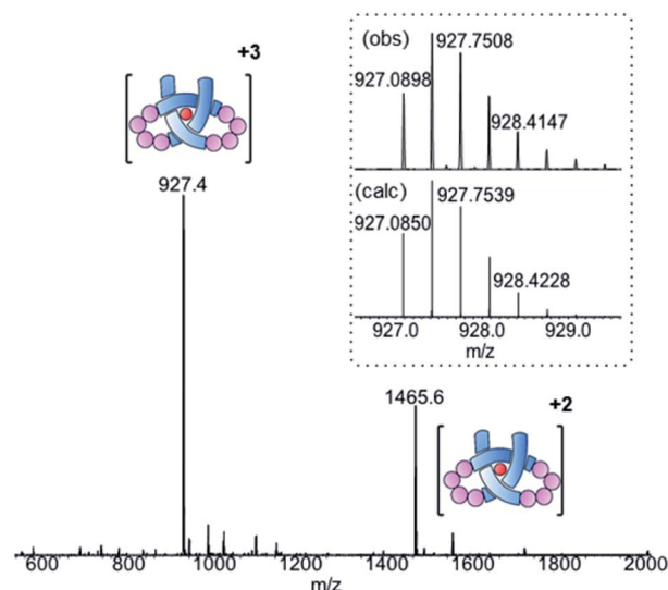
Fig. 4 ESI-MS (positive mode) of pseudopeptide overhand knot complex 8\cdot[\text{Lu}] . Inset: isotopic distribution for [\text{M}]^{3+} signal from HR-MS.
