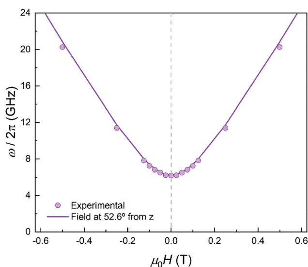
Fig. 10 Experimental effective energy gap \hbar\omega = k_B T_0/0.42 , with T_0 the field-dependent temperature of the heat capacity maximum. The solid line shows the behaviour expected for a magnetic field applied at 52.6^\circ from the anisotropy axis.
