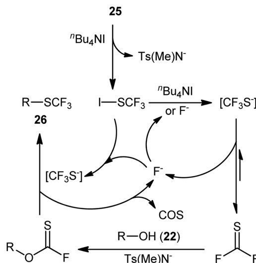
Scheme 16 Proposed pathway of alkyl trifluoromethylthioethers 25 formation.
