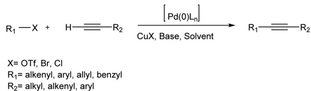
Scheme 1 The Sonogashira reaction structure.
