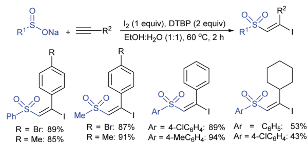
Scheme 125 \text{I}_2 -mediated iododisulfonation of alkynes using sodium sulfinates.
