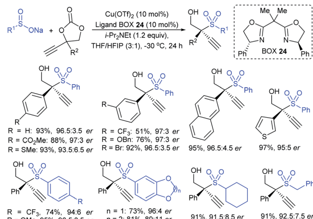
Scheme 68 The Cu-catalyzed asymmetric sulfonylation of propargylic cyclic carbonates with sodium sulfinates.
