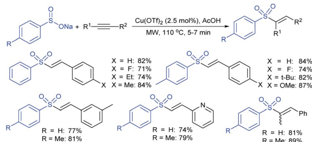
Scheme 93 \text{Cu(OTf)}_2 -catalyzed hydrosulfonylation of alkynes with sulfonates.
