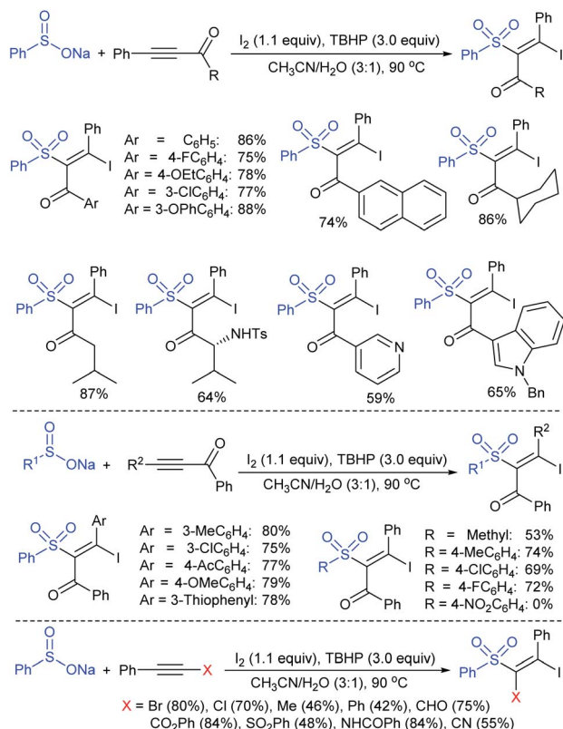
Scheme 126 Iodine-mediated iodosulfonylation between activated internal alkynes and sodium sulfinates.
