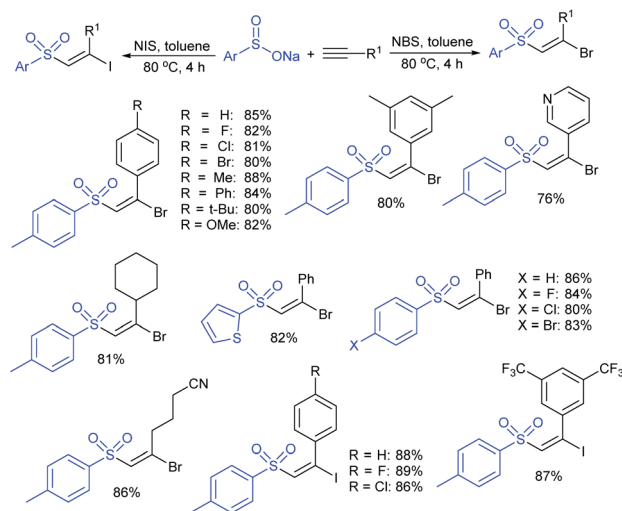
Scheme 123 NBS/NIS-mediated halosulfonation of alkynes using sodium sulfinates.
