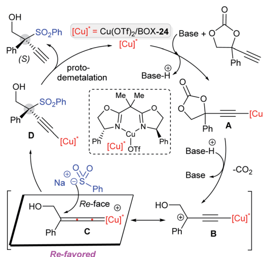
Scheme 69 Mechanism for the Cu-catalyzed asymmetric sulfonylation of propargylic cyclic carbonates with sodium sulfinates.
