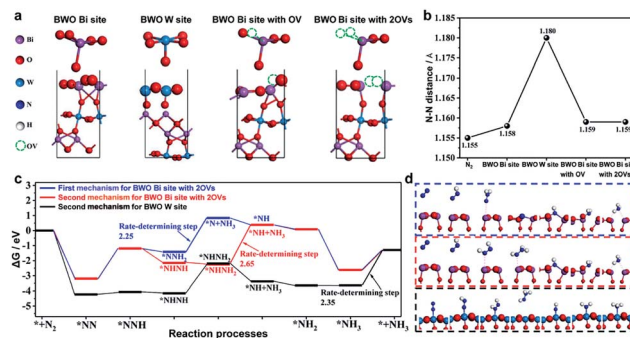
Fig. 27 (a) Models of the four possible active sites for Bi 2 WO 6 (010) surface, W site, Bi site, Bi site with OV, and Bi site with 2OVs. (b) N–N distance of free N 2 and N 2 on the four possible active sites. (c) Gibbs free energy during the reaction processes via two different mechanisms (the first mechanism: * + N 2 → *NN → *NNH → *NNH 2 → *N + NH 3 → *NH → *NH 2 → *NH 3 → * + NH 3 and the second mechanism: * + N 2 → *NN → *NNH → *NNH 2 → *NHNH 2 → *NH + NH 3 → *NH 2 → *NH 3 → * + NH 3 , where * represents the active site) and (d) the free-energy profile of three possible processes for BWO W site and BWO Bi site with 2OVs. Reprinted with permission from ref. 100 Copyright 2021, the American Chemical Society.
