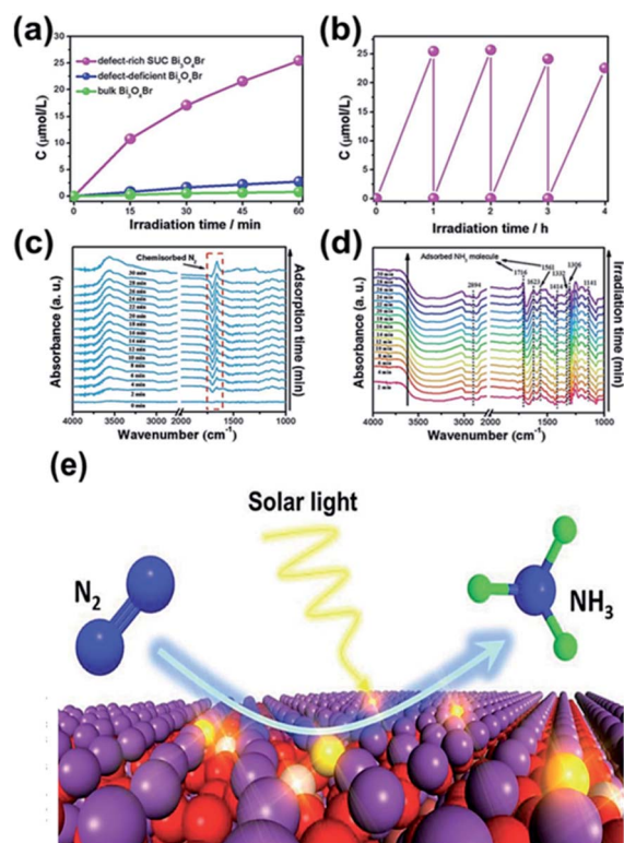
Fig. 9 (a) Quantitative evaluation of NH_3 generated and (b) stability of defect-rich SUC Bi_3O_4Br under light irradiation. (c) In situ FTIR spectra of SUC Bi_3O_4Br catalysts during N_2 adsorption without irradiation (c) and under irradiation (d). (e) Scheme of the photocatalytic N_2 fixation process. Reprinted with permission from ref. 99 Copyright 2019 Wiley-VCH.
