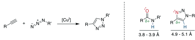
Scheme 32 Left: reaction scheme of the \text{CuI} -catalyzed azide–alkyne cycloaddition. Right: comparison of electronic and steric properties of the Z -amide and the 1,4-substituted 1,2,3-triazole. Red: H-bond acceptor position, blue: H-bond donor position.
