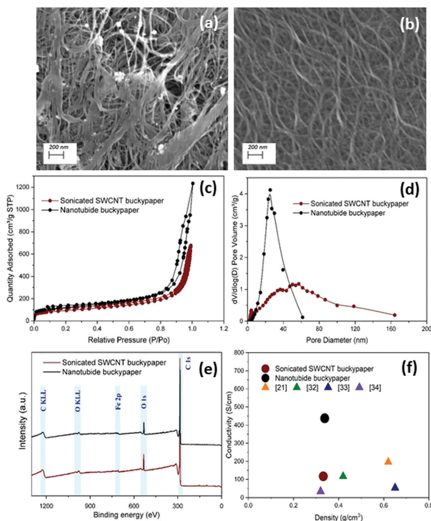
Fig. 1 SEM images of (a) sonicated SWCNT buckypaper and (b) nanotubide buckypaper ( [C] = 1.5 \text{ mg ml}^{-1} , C : Na = 10 : 1 ). Comparison of sonicated SWCNT buckypaper and nanotubide buckypaper ( [C] = 1.5 \text{ mg ml}^{-1} , C : Na = 10 : 1 ) by (c) BET N_2 adsorption-desorption isotherms, (d) pore size distribution (PSD) and (e) XPS survey scans. (f) Electrical conductivity of nanotubide and sonicated SWCNT buckypapers compared to other SWCNT buckypapers in the literature. 21,32–34
